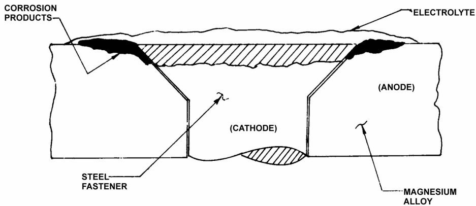
Galvanic corrosion occurs when two dissimilar metals make contact in the presence of an electrolyte. (See figure at left.) It is usually recognizable by the presence of a build-up of corrosion at the joint between the metals. (Diagram: Aviation Safety Bureau)
